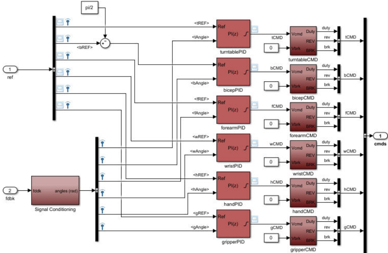
Figure 3: Controller structure.
