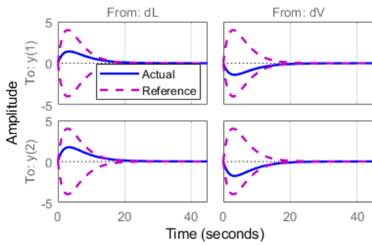
Requirement 3: Step disturbance rejection
